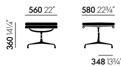
Soft Pad Chair EA 223, Taburete, no giratoria
