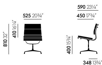
Soft Pad Chair EA 205 (nueva altura), no giratoria, sin reposabrazos
