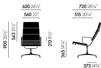
Soft Pad Chair EA 215, no giratoria, con reposabrazos
